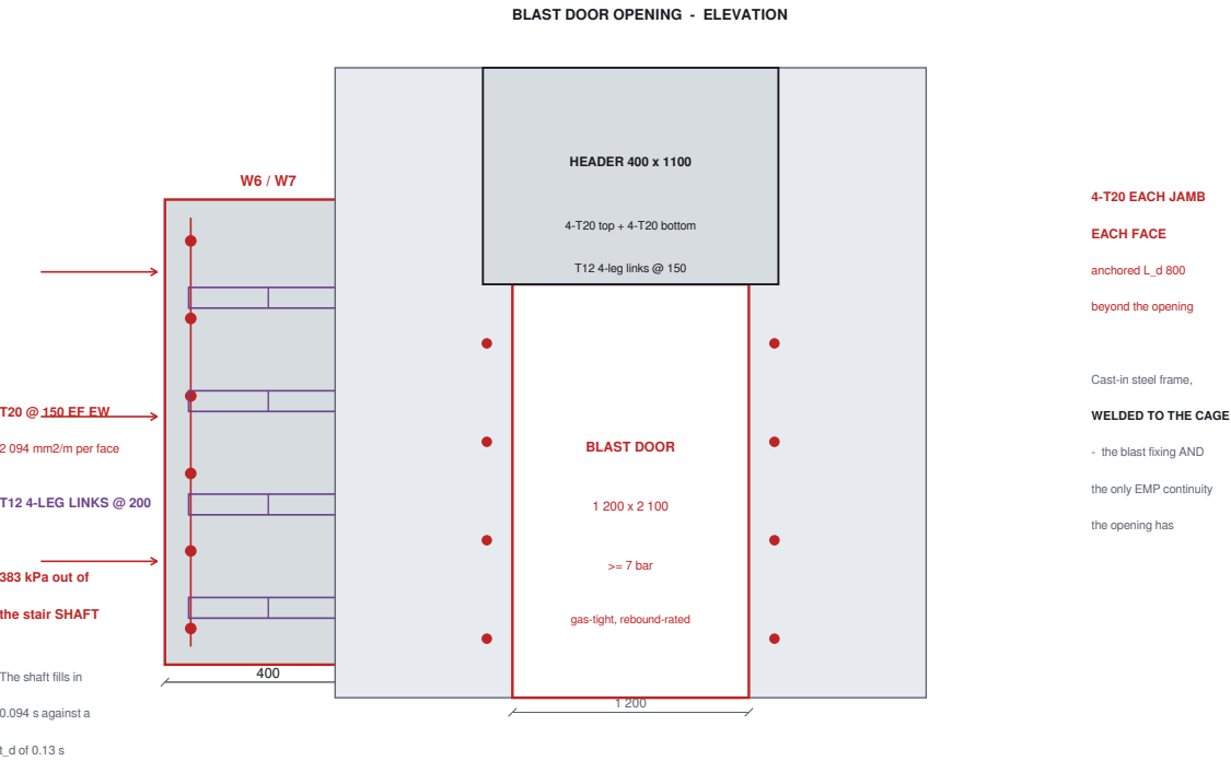
Figure 26 Walls W6 and W7 at 400, and the blast door openings they carry.
