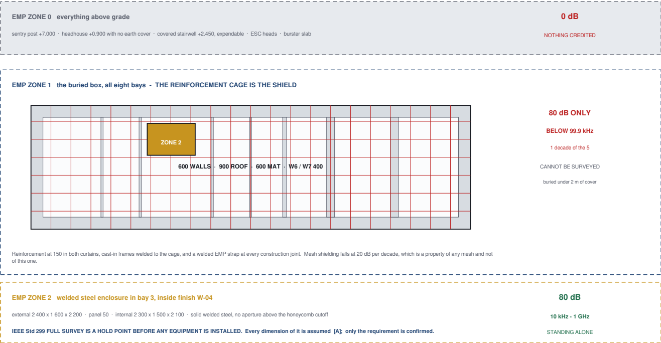
Figure 46 The three EMP zones, and the one that carries the requirement.
