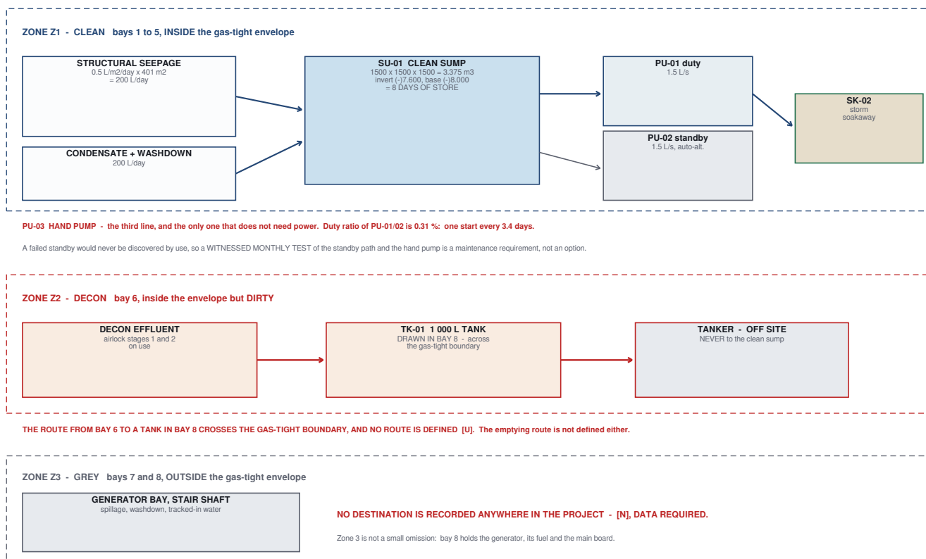
Figure 42 The three hydraulic zones, and the one that has nowhere to go.
