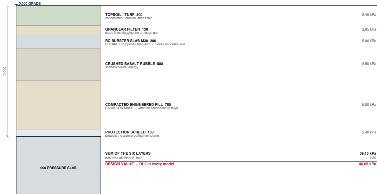
THE ENGINEERED COVER - 2 000 mm IN SIX LAYERS
