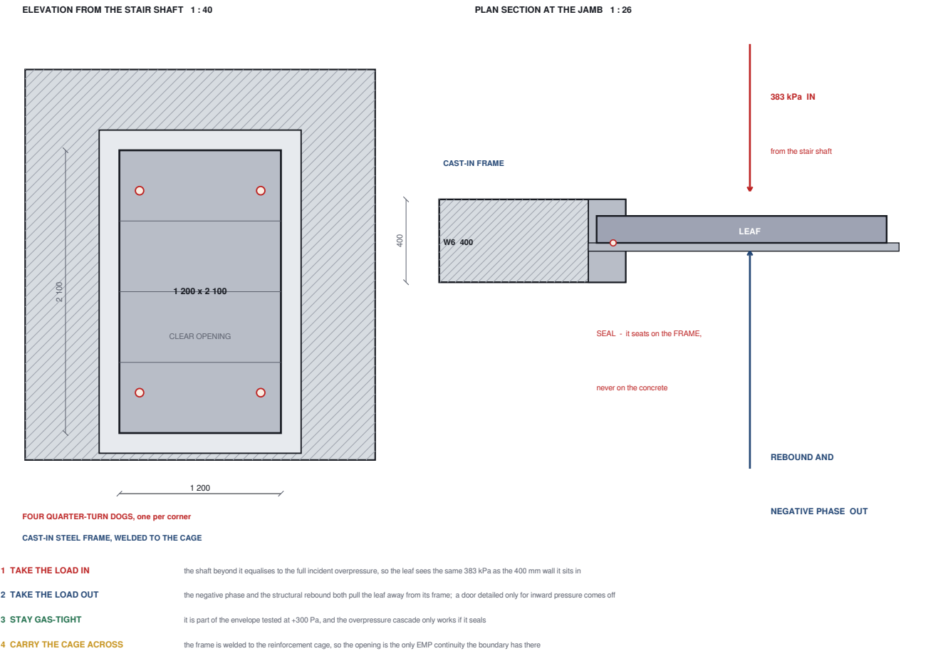
Figure 32 Blast door 1 in W6 - elevation, jamb section, and the four things the closure has to do at once.
